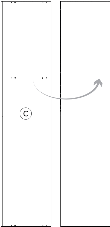
CA04268 1828x407x16mm
