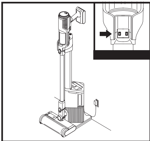
CHARGING WHILE IN STORAGE MODE
