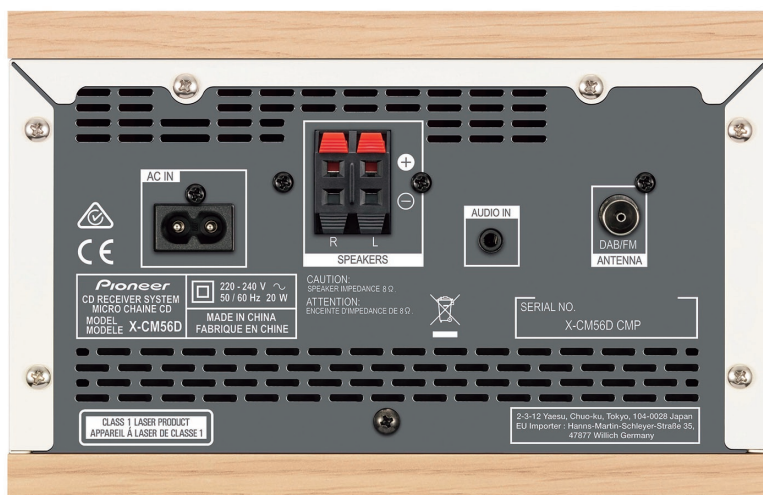
X-CM56D(W)/CMP
